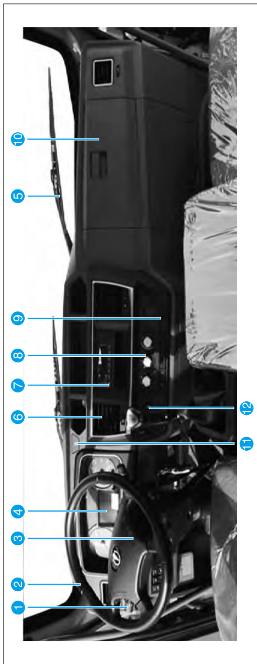
仪表及操纵机构的布置
